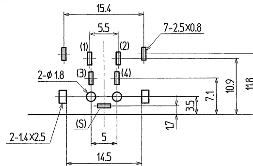
Dimensions of PC board holes/参考基板孔配置図 (t=1.6) (Tolerance/公差 ALL±0.1)(Parts side view/部品面より見る)
