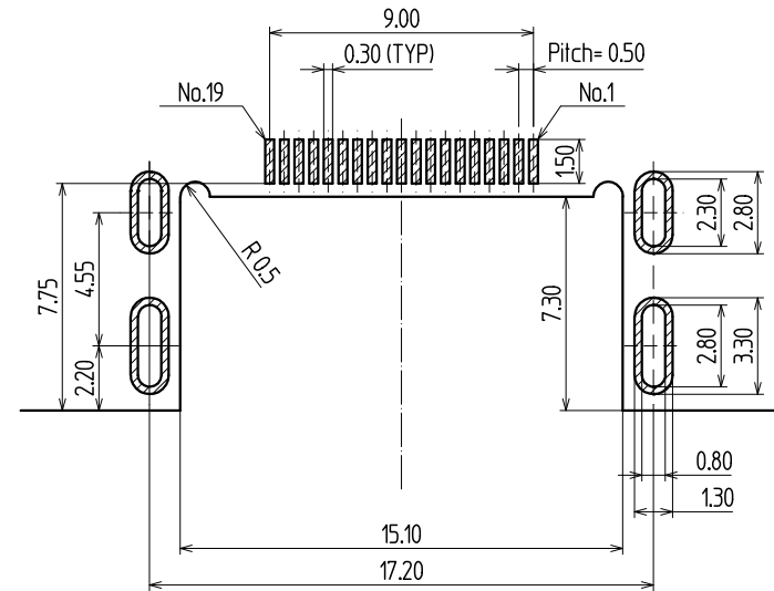
Dimensions of P.C.B layout
