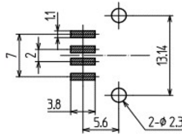
Dimension of P.C.B Layout(Parts Side View)
