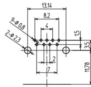
Dimensions of PC board holes (Parts side view)
