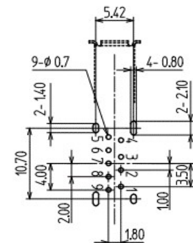
Dimensions of PC board holes (Parts side view)
