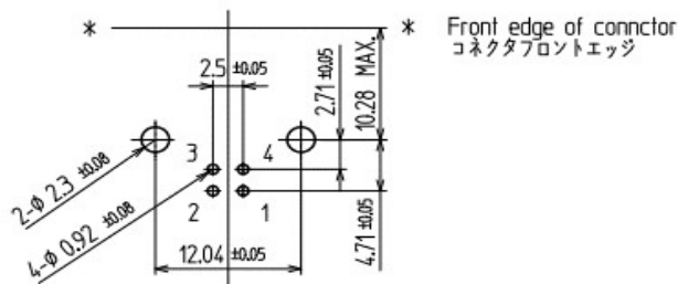
t1.6 Dimensions of PC board holes (Tolerance all±0.1, Dip-side view)
