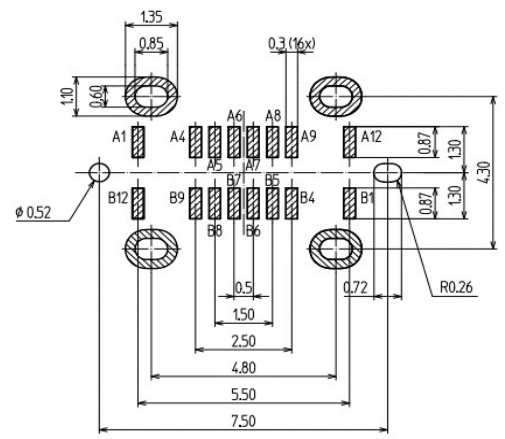
PC BOARD LAYOUT/参考基板孔寸法図 (S=10/1) (Tolerance/公差 ALL±0.05)(Parts Side/部品面)
