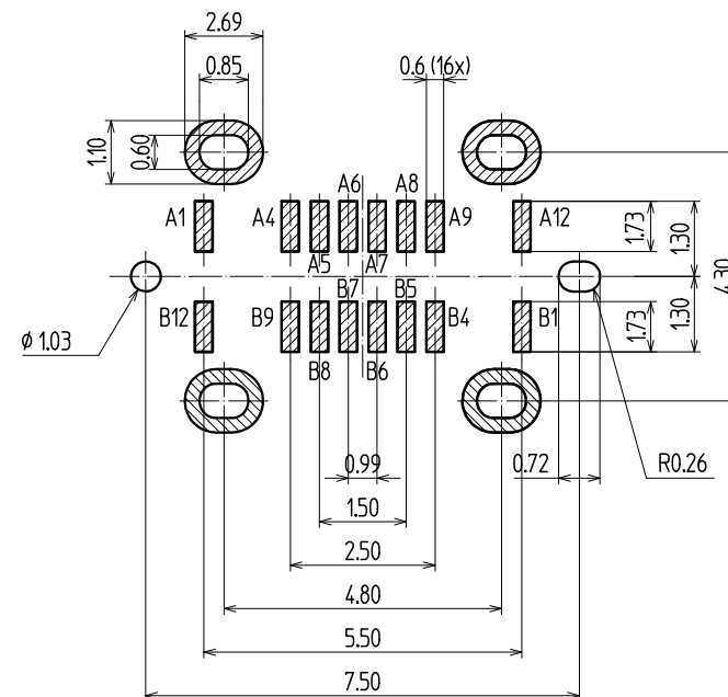
PC BOARD LAYOUT/参考基板孔寸法図 t0.8 (S=10/1) (Tolerance/公差 ALL±005)(Parts Side/部品面)
