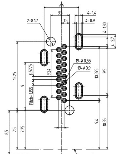
Dimensions of PC board holes / 参考基板孔寸法図
