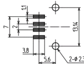
Dimension of P.C.B Layout(Parts Side View)
