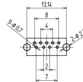
Dimensions of PC board holes (Parts side view)
