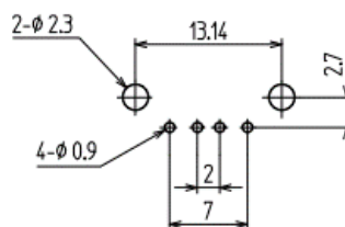
Dimensions of PC board holes 参考基板孔寸(Tolerance/公差 ALL ±0.05)
