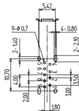
Dimensions of PC board holes (Parts side view)
