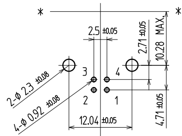
t1.6 Dimensions of PC board holes (Tolerance all±0.1, Dip-side view)
