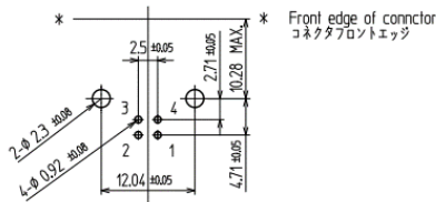
H1.6 Dimensions of PC board holes (Tolerance all±0.1, Dip-side view)
