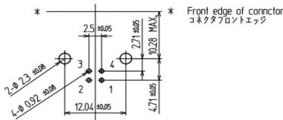
H1.6 Dimensions of PC board holes (Tolerance all±0.1, Dip-side view)
