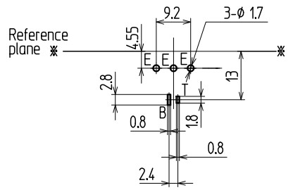
Referential dimensions of PC board holes 参考基板孔寸法図 (Tolerance/公差 ALL±0.1) (Printed-side view/パターン側) t1.6
