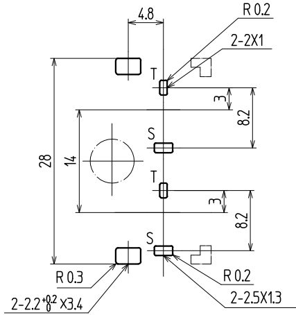
Referential dimensions of PC board holes / 参考基板孔寸法図 (Printed-side view/パターン面)(Tolerance/公差 ALL±0.1)1/6
