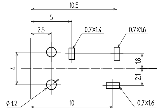
Dimensions of PC board holes / 参考基板孔
