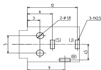
Dimensions of PC board holes/参考基板孔 Parts side view/部品面より見る Tolerance/公差 ALL±0.1
