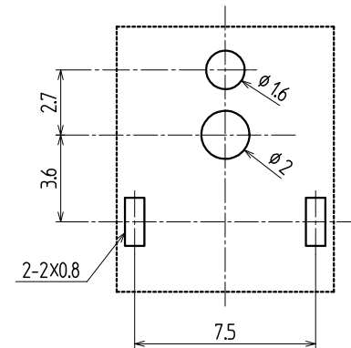
Dimensions of PC board holes/参考基板孔 Parts-side view/部品側 Tolerance/公差 ALL±0.1
