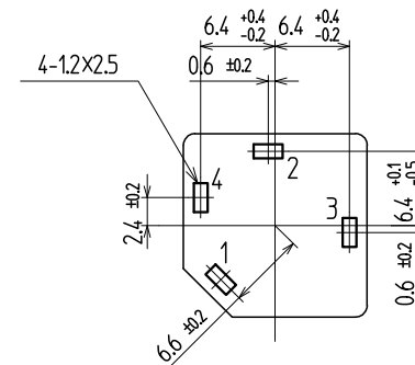
Referential dimensions of PC board holes/参考基板孔寸法図 (Parts-side view/部品面) (S=2/1)
