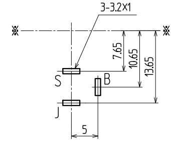
Dimensions of PC board holes / 参考基板孔
